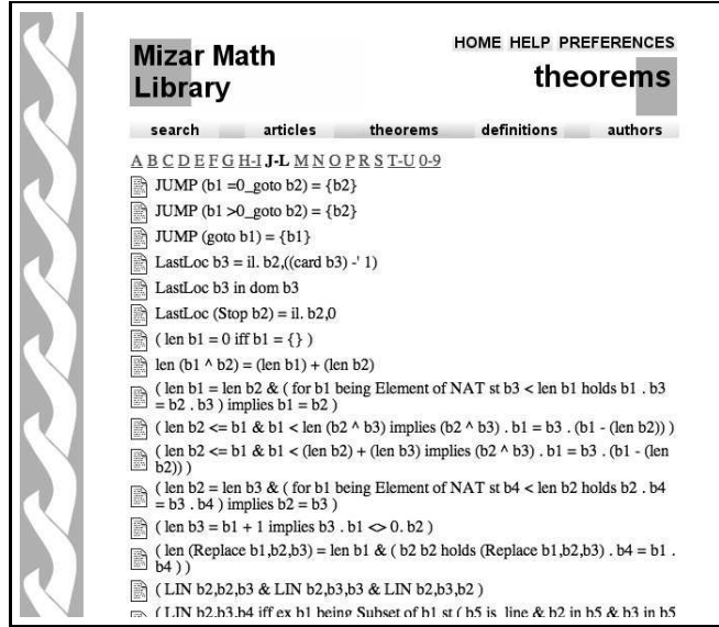
Fig. 3. Browsing the theorem list in the Mizone
